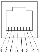
PD and PSE Eight-Pin RJ45 Modular Jack
